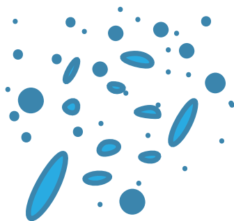
Water droplets in the cloud
